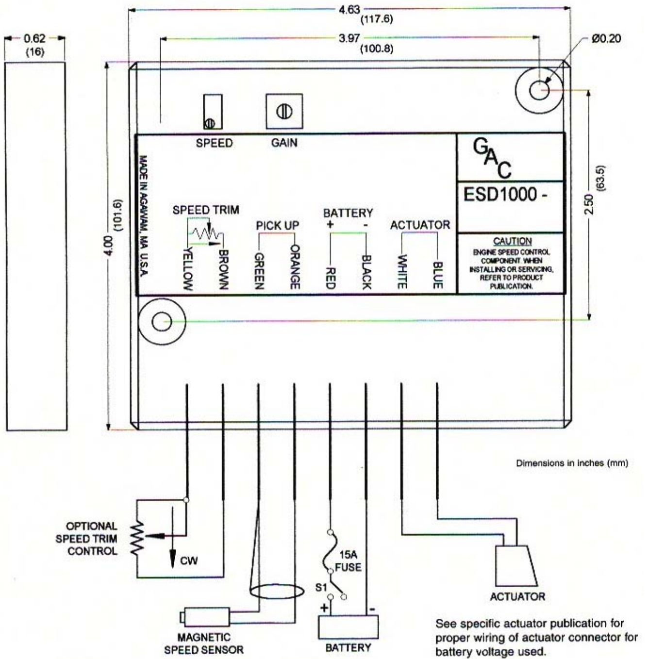
Diagram 1. SYSTEM WIRING/OUTLINE
